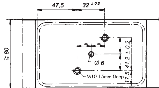
location of mounting holes and fill connection
