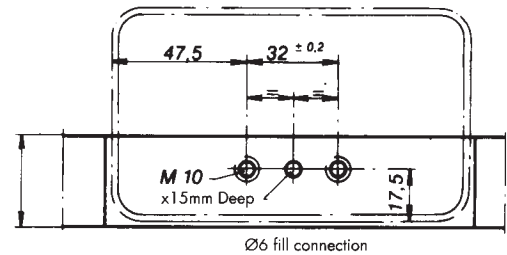
location of mounting holes and fill connection
