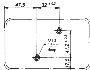
location of mounting holes
